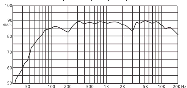
DSP6608 Frequency Response (dB SPL, 1W, 1m)
