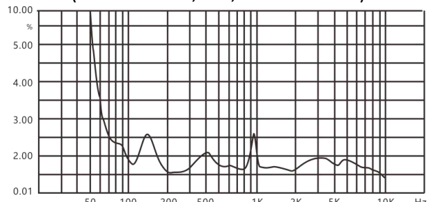
DSP6608 Distortion (THD< 5% 1W, 1m, 100Hz-10kHz)
