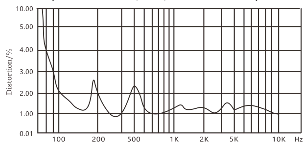
DSP6606 Distortion (THD< 5% 1W, 1m, 100Hz-10kHz)
