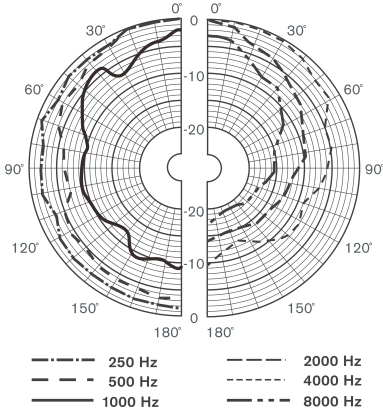
DSP6606 Horizontal Directivity Pattern
