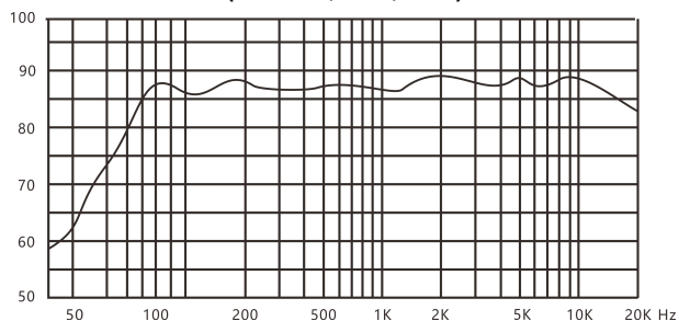
DSP6606 Frequency Response (dB SPL, 1W, 1m)
