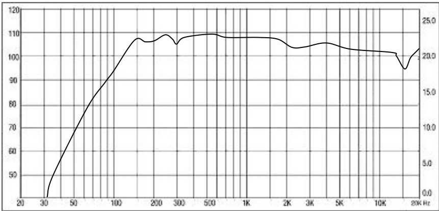
Product Frequency Response (dB SPL, 1W, 1m)
