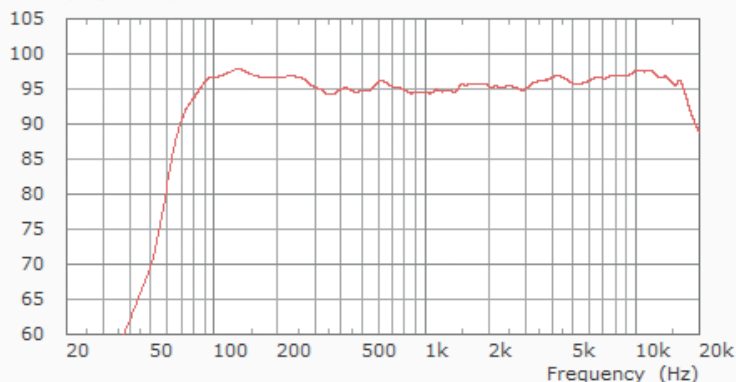
(dB) Level, SPL 1W 1m VLX12
